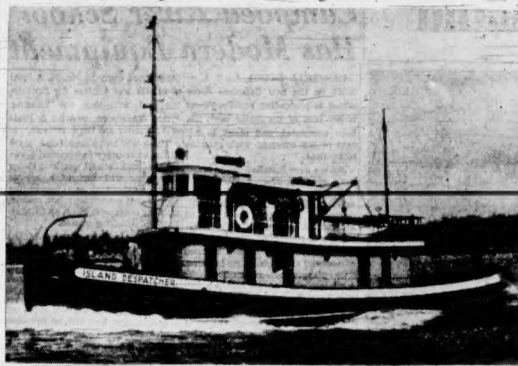
Latest addition to the large tug fleet of Island Tug & Barge Ltd. is 85-foot Island Despatcher, pictured above during recent trial runs. She is powered with 320-horsepower Atlas Imperial engine, and brings to 14 number of towing craft operated by local firm. Island Despatcher's first job was removal of packer, Ribac from Sidney Spit last Tuesday night.
